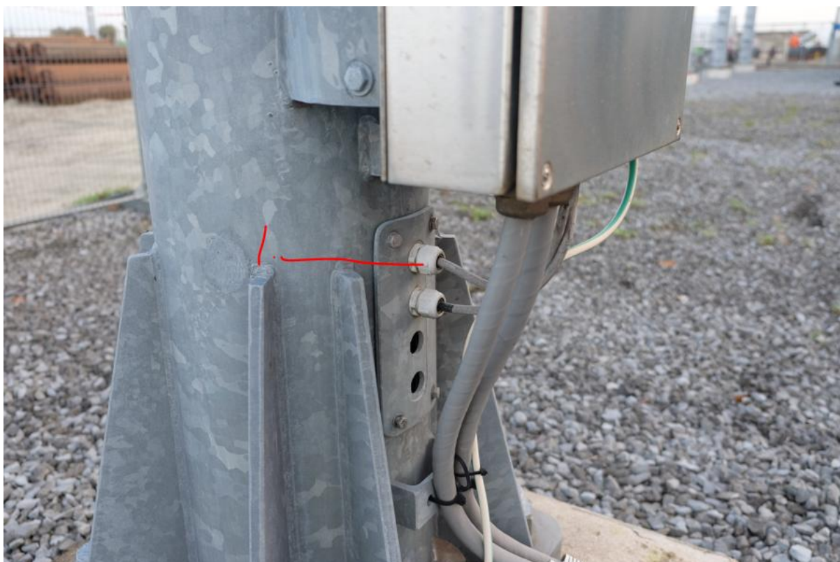
2. SMH051 (Appears to be plastic connectors that are not EMC compliant).
